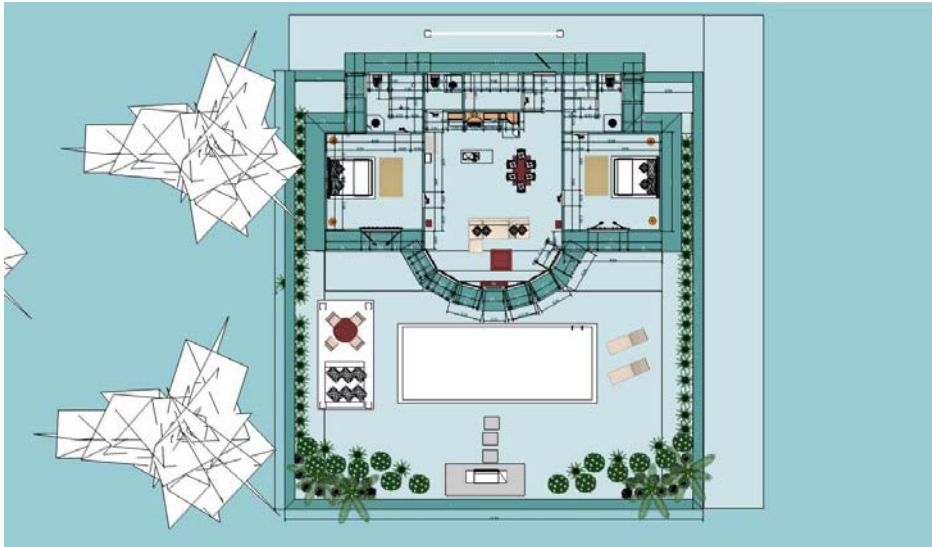
Floor plan 2-bedroom
